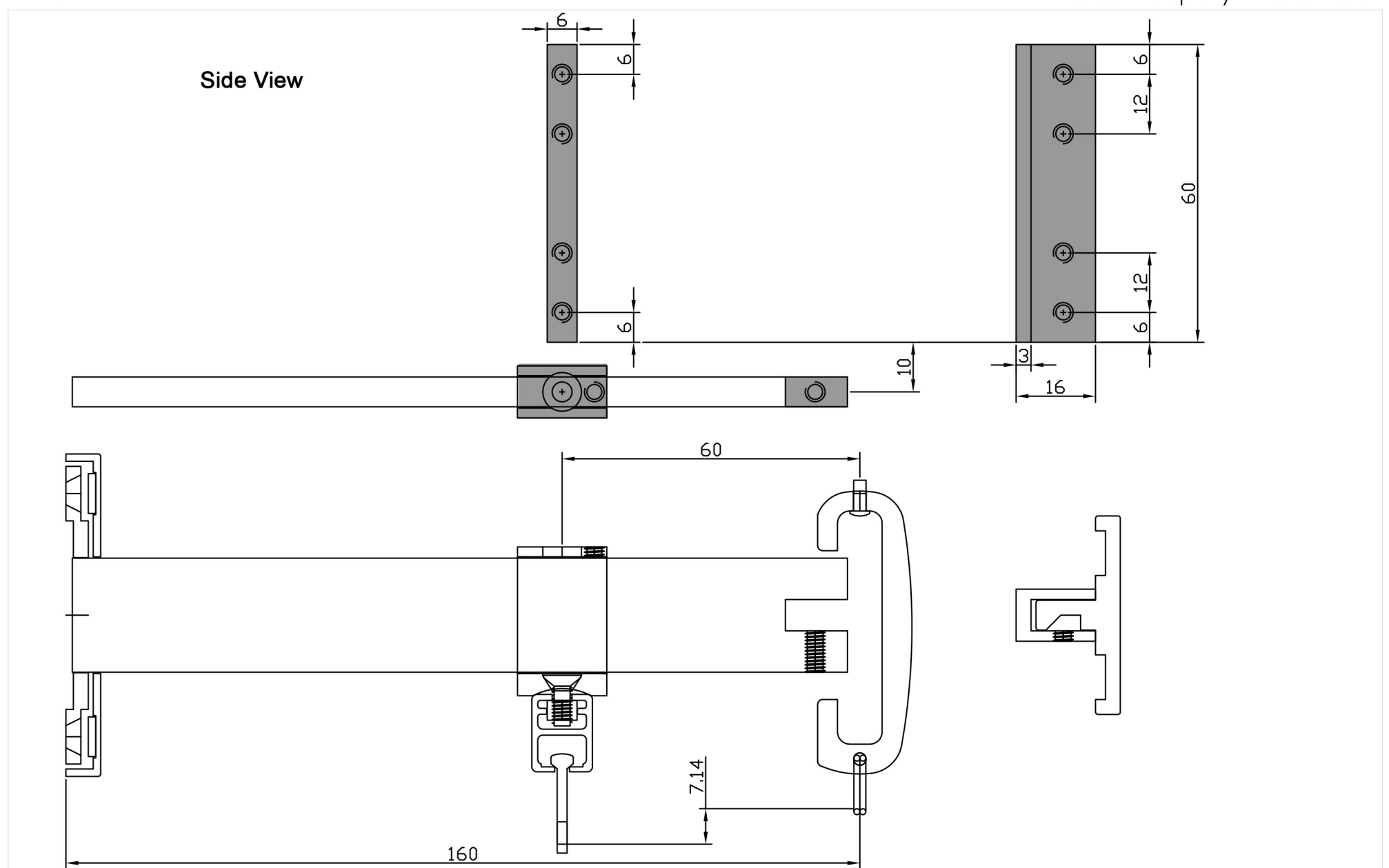
SHOWN: 2 Piece Double Bracket Center Splice DMX43/STL.
